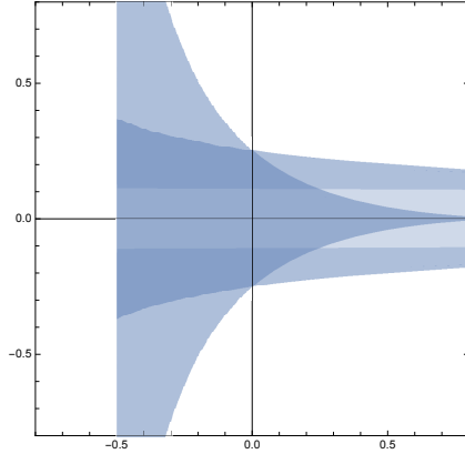
Figure 3: Image of \mathbb{D} under C_{1, z/(1-z^2)}[z/(1-z)]
