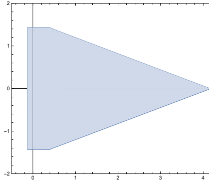
Figure 4: Image of \mathbb{D} under C_{10, L_{-1}}[f_2]
